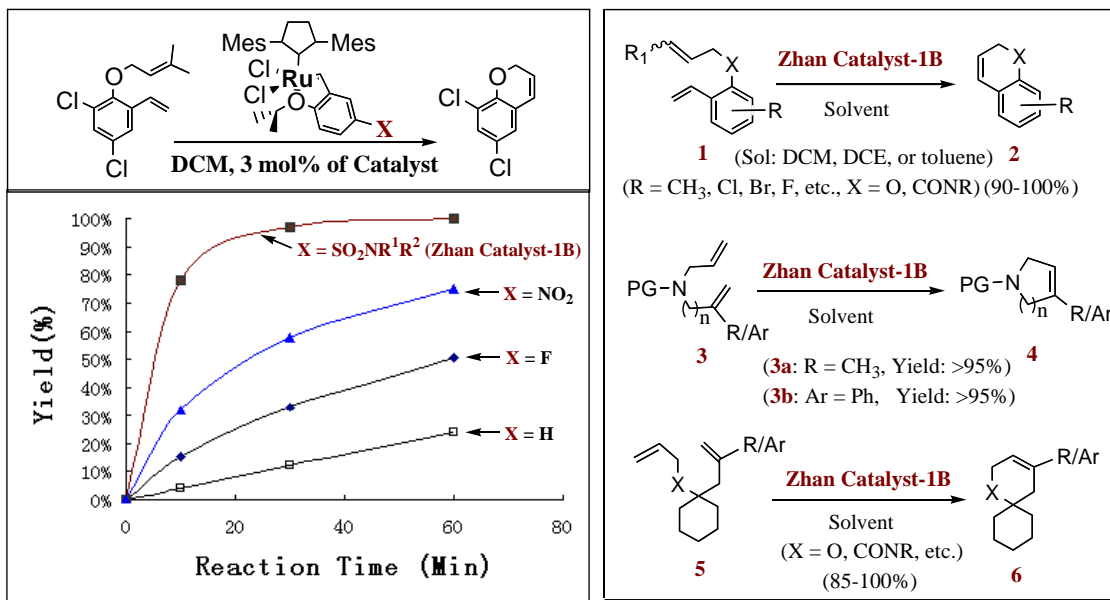
Fig. 1. Comparison of Four Ru Catalysts for RCM
